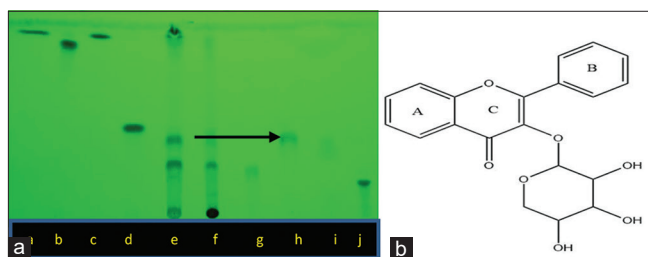
Figure 5: (a) TLC co-chromatography of DE and DEA with standard compounds: a. kaempferol, b. quercetin, c. apigenin, d. gallic acid, e. DEA, f. DE, g. chlorogenic acid, h. quercitrin, i. luteolin 7-O glycoside, j. rutin, monitoring under UV light \lambda 254 nm; (b) quercitrin structure
