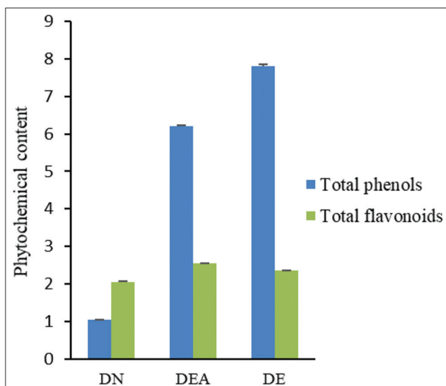
Figure 3: Phytochemical content of Pouteria campechiana leaves extract
