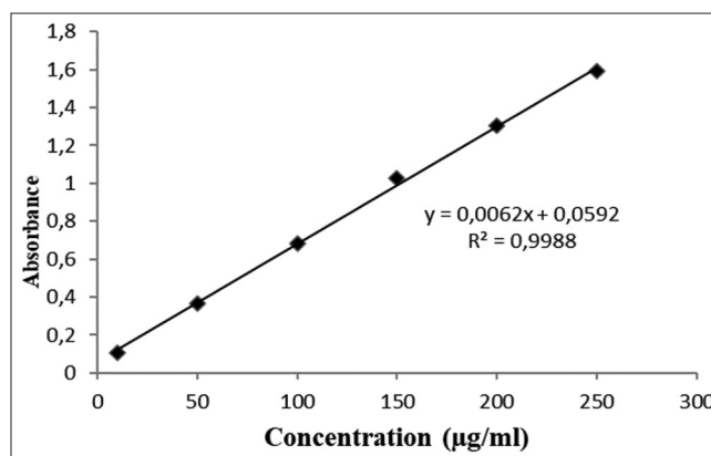
Figure 1: Calibration curve of gallic acid
