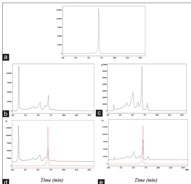
Figure 6: (a) Chromatogram HPLC of quercitrin; (b) DE; (c) DEA; (d) overlay quercitrin with DE; (e) overlay quercitrin with DEA
