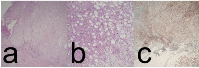
Figure 3: Histopathology of the dermal pleomorphic sarcoma (Case 2); a) Overview (hematoxylin-eosin x 2); b) Deep infiltration in the subcutaneous adipose tissue (hematoxylin-eosin x 4); c) Expression of CD10 (x 2)
