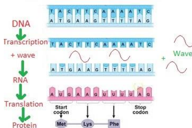
Figure 2: During transcription and translation, electrical pairs become separated, and some waves emerge
