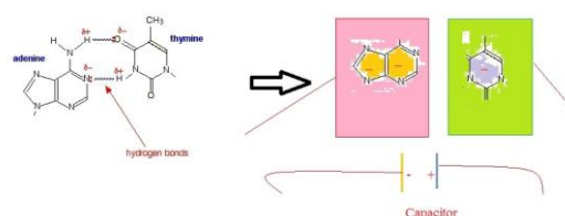
Figure 1: A capacitor is formed from Adenine and Thymine
