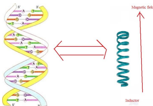
Figure 3: Each gene is coiled several times, and its structure is similar to an inductor
