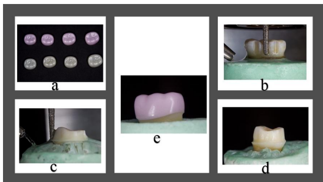
Figure 1: a) Nusmile prefabricated zirconia crown and their counterpart pink try-in crown for lower left 2nd primary molars (Houston, TX, USA), b) depth cuts to determine facial and lingual reduction, c) Showing step of removing of the depth cuts to complete preparation for zirconia crown using a special milling machine mounted with coarse tapered stone, d) after removing all depth cuts leaving an edge all around tooth, e) Showing Try in step: the pink try-in crown is the same size as its tooth-coloured counterpart and was used to accurately determine correct passive fit after smoothing and polishing the anticipated edge to a feather edge
