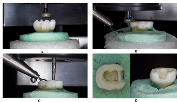
Figure 2: A) showing occlusal depth cuts for occlusal reduction of endocrown preparation, B) showing mounted wheel stone on conventional-speed straight hand-piece attached to the milling machine was reducing occlusal surface with coolant to produce a flat cervical sidewalk, C) showing a mounted tapered stone of 8-degree angle during flaring of axial wall for the axial preparation of endocrown, D) showing final tooth preparation for endocrown restoration with "cervical sidewalk" after smoothing and polishing the walls
