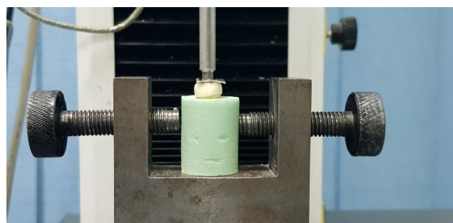
Figure 5: Showing fracture test done by compressive mode of load applied occlusally using a metallic rod with a round tip (3.6 mm diameter) using a universal testing machine
